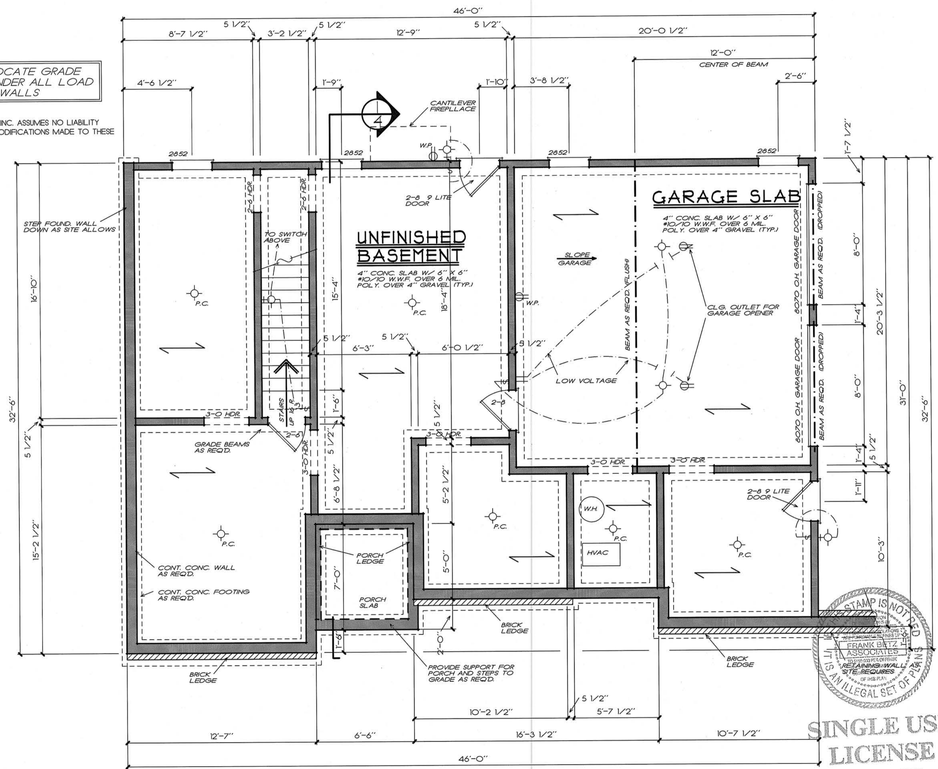
BASEMENT FOUND. PLAN 1/4" = 1'-0"
